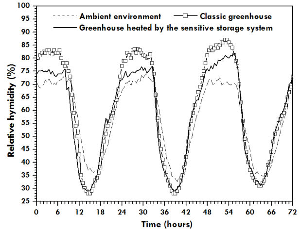
Figure 9. Relative humidity variation inside the classic greenhouse, the experimental greenhouse and the outdoor environment
