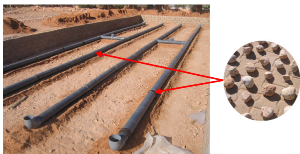
Figure 2. PVC tubes in H-shape filled with rocks
