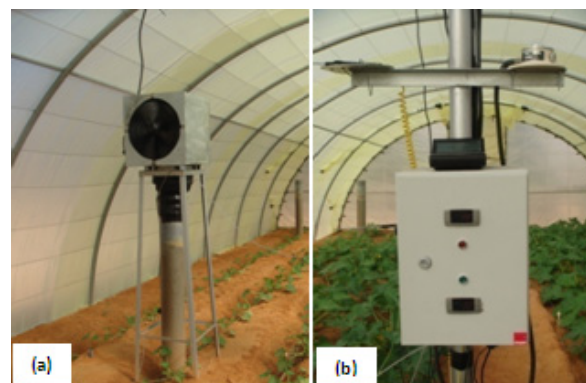
Figure 4. (a) Fan; (b) Smart temperature control system
