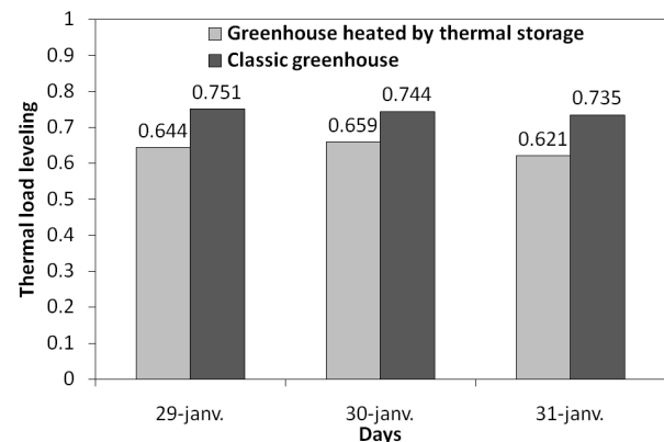
Figure 12. Thermal load leveling of experimental and classic greenhouse
