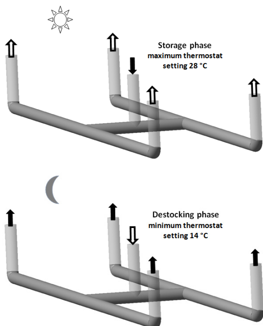
Figure 5. Operating principles of the rock-bed heating system
