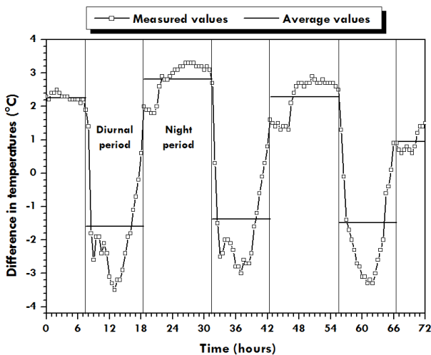
Figure 8. Air temperature gaps inside both experimental and classic greenhouse
