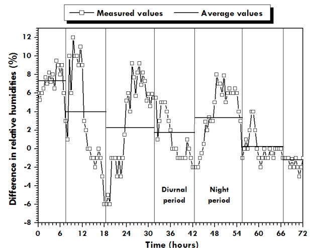
Figure 10. Relative humidity gaps inside experimental and classic greenhouses
