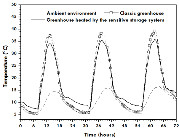
Figure 7. Air temperature variation with time of outside/inside greenhouse with and without heating
