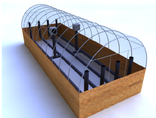
Figure 3. A rock-bed heating system in a greenhouse
