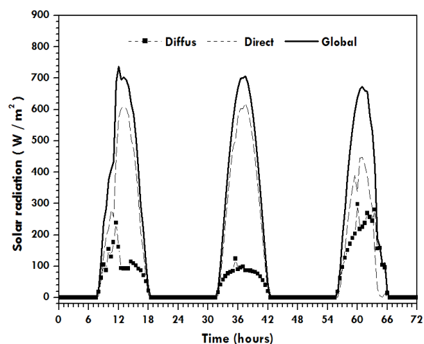
Figure 6. Evolution of solar radiation outside the greenhouse
