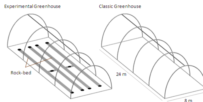
Figure 1. Schematic view of the studied greenhouses
