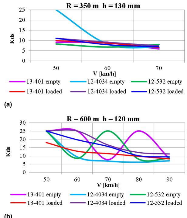
Figure 12. Variation of the safety factors of the wheel against derailment with the motion speed: (a) R=350 m curve; (b) R=600 m curve
