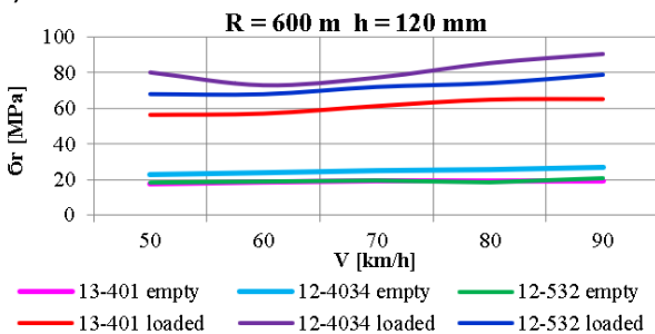
Figure 17. Variation of the edge stress in the rail base with the motion speed: (a) R=350 m curve; (b) R=600 m curve
