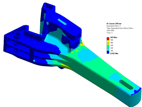
Figure 2. Equivalent stress distribution field, compression, displacement of the axis of an adjacent automatic coupling 0.1 m higher than the considered, MPa
