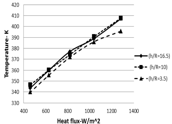
Figure 13. Mean surface temperature versus heat flux with different depth/radius ratios.
