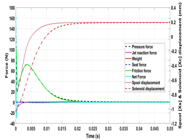
Figure 7. Forces acting on the valve's spool at 7V
