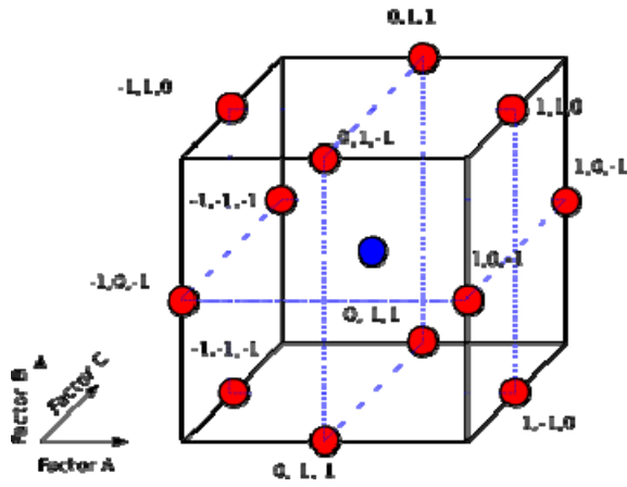
Figure 1. Box-Behnken design
