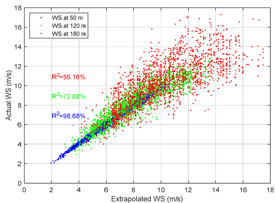
(g) ER Extrapolated WS Scatter Plot
