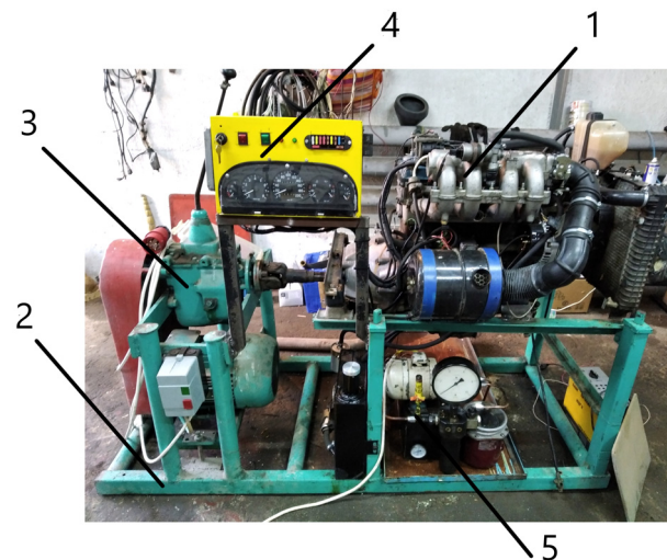
Figure 5. Experimental setup: 1– ZMZ-4062 engine; 2– stand frame; 3– electric transmission; 4– remote control; 5– oil hydraulic system for turbocharger power supply.
