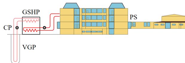
Figure 4. Scheme of GSHP in the PS
