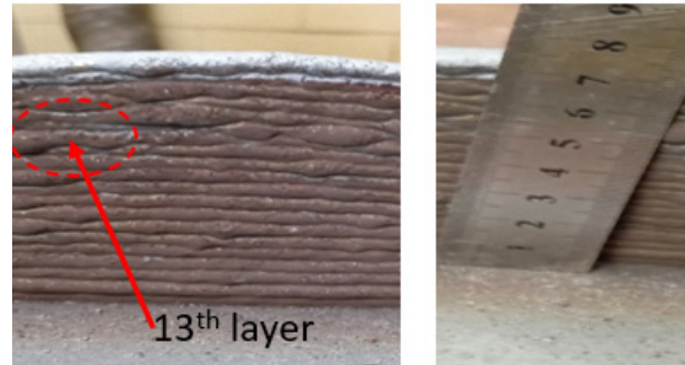
Figure 12. Appearance of 20 layers single pass wall for 316L
