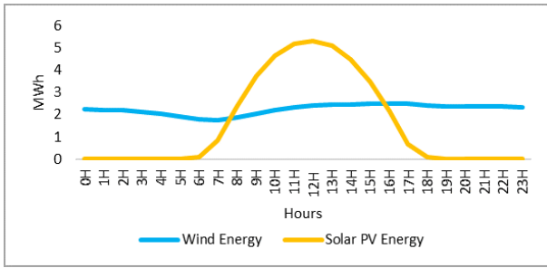
Figure 8. Average Monthly estimation of hourly energy generation for idevedual solar PV block and wind turbine
