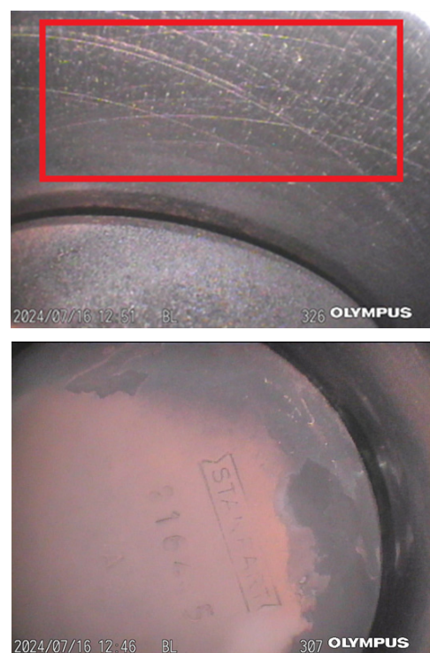
Figure 6. Endoscope image about the cylinder liner (above) and piston (below) of the investigated Triumph SC 1300 engine.
