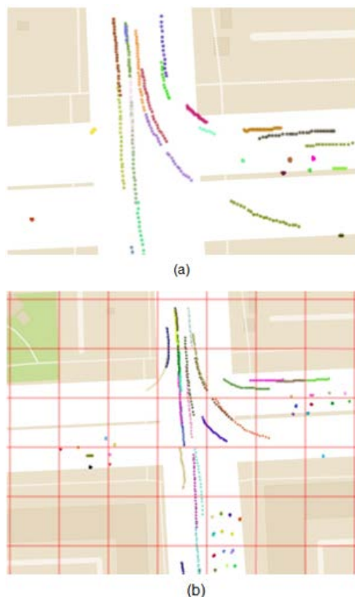
Figure 8. (a) Queues of vehicle detections with a frequency of 3 seconds; (b) Breakdown of detections into 20×20 meter cells
