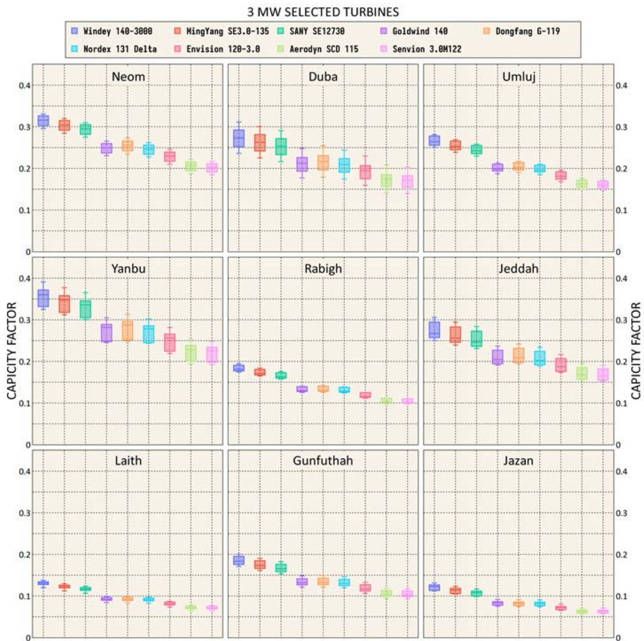
Figure 9. Capacity factor for 9 selected 3 MW turbines for all selected sites
