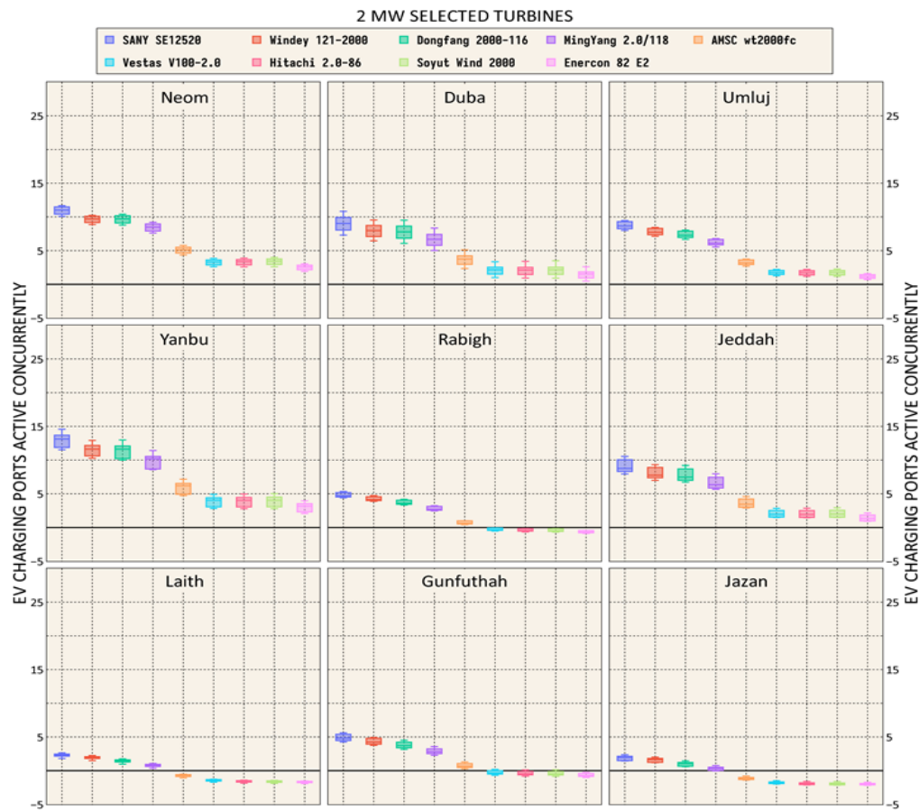
Figure 12. EV charging ports active concurrently using 9 selected 2 MW turbines for all selected sites. (negative value implies insufficient wind turbine power to run auxiliary systems at EV charging stations)
