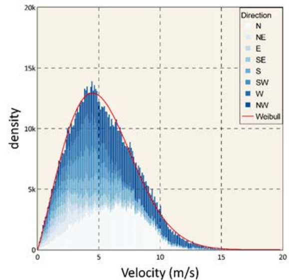
Figure 2. Weibull distributions for wind speeds
