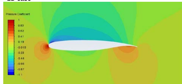
Figure 13. Pressure coefficient – NASA sc (2) 0712 at AOA 0° - 3D case
