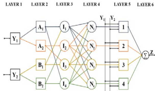
Figure 2. ANFIS Architecture
