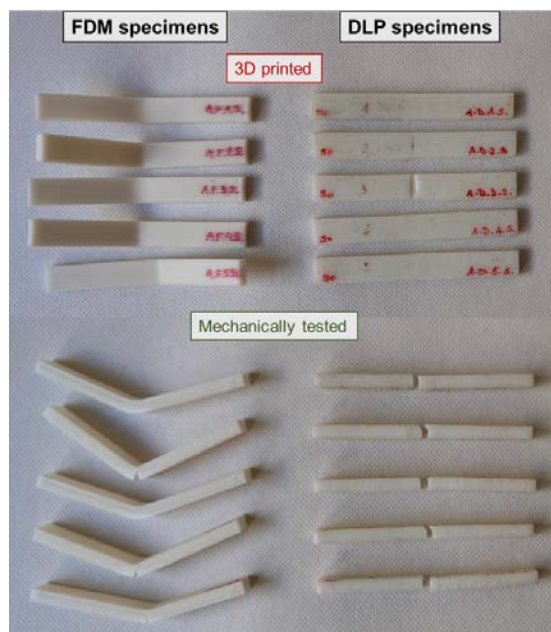
Figure 2. 3D printed and mechanically tested specimens.
