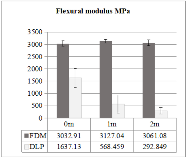
Figure 6. Flexural Modulus for aging specimens made by FDM and DLP-LCD technology.
