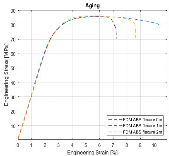
Figure 4. Stress-strain curves for aging specimens made by FDM technology.
