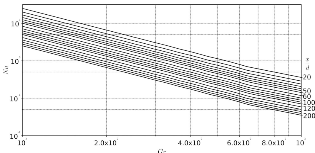
Figure 8. A nomogram of the Nusselt number dependence on the Grashof number for values of x/d ranging from 20 to 200
