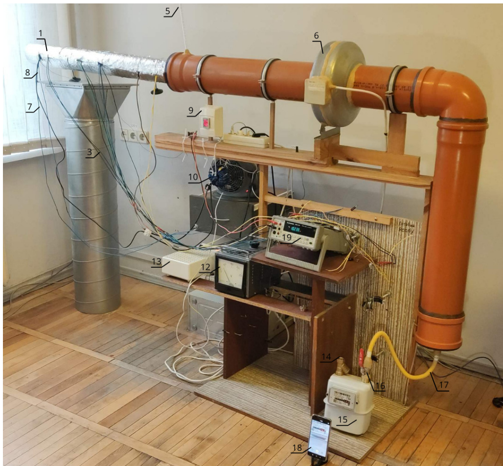
Figure 4. Experimental setup for determining local heat transfer coefficients from the channel surface to air
