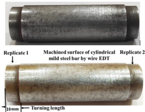
Figure 3. 3D view with detailed specifications of a cylindrical mild steel bar after precision straight turning on both ends by wire-EDT.
