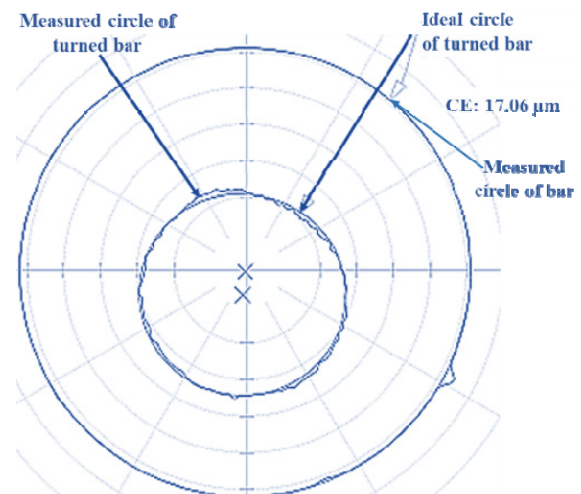
Figure 7. Circularity error in the geometrical profile of mild steel bar after turning at an optimum combination (i.e. run 3) by wire-EDT.
