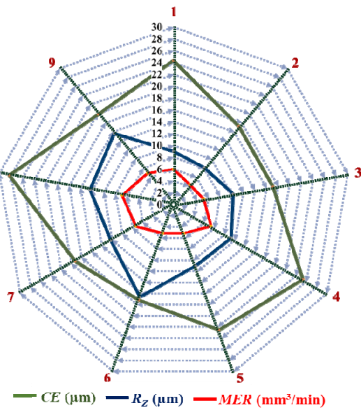
Figure 5. Variation in circularity error; mean surface irregularity depth; and machining erosion rate with machining combinations.
