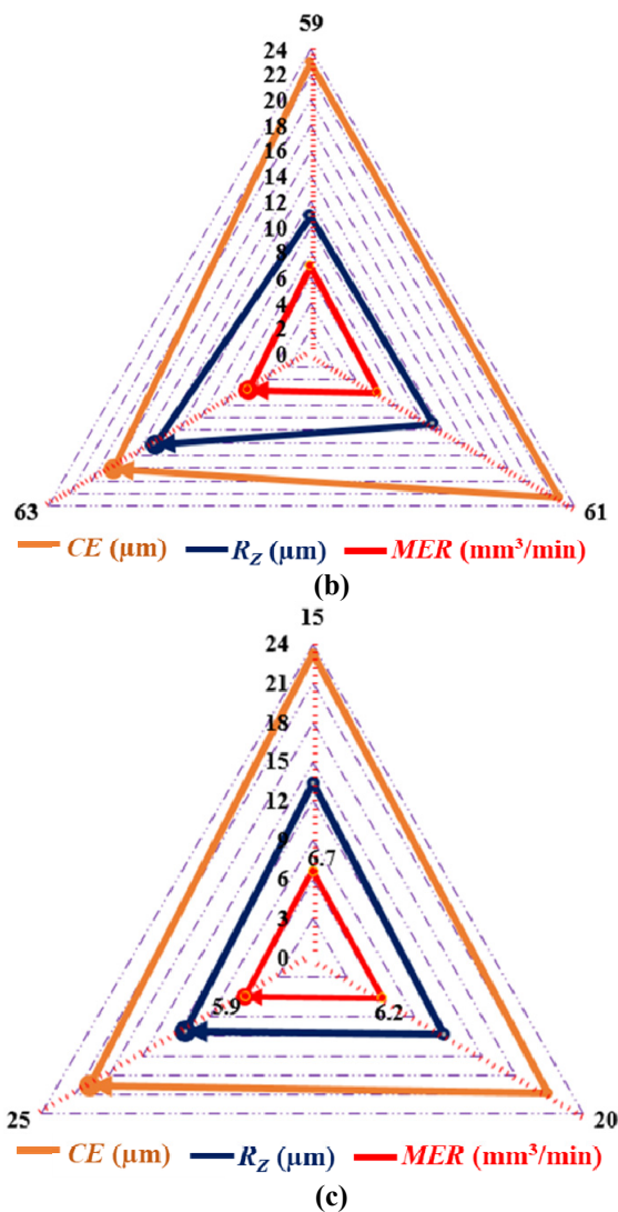
Figure 6. Variation in CE , R_z , and MER with (a) pulse-on duration; (b) pulse-off duration; and (c) servo voltage.
