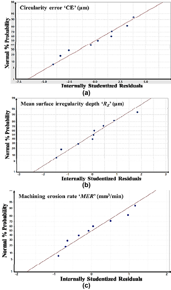
Figure 4. Normal probability graphs of selected responses: (a) circularity error; (b) mean surface irregularity depth; and (c) machining erosion rate.
