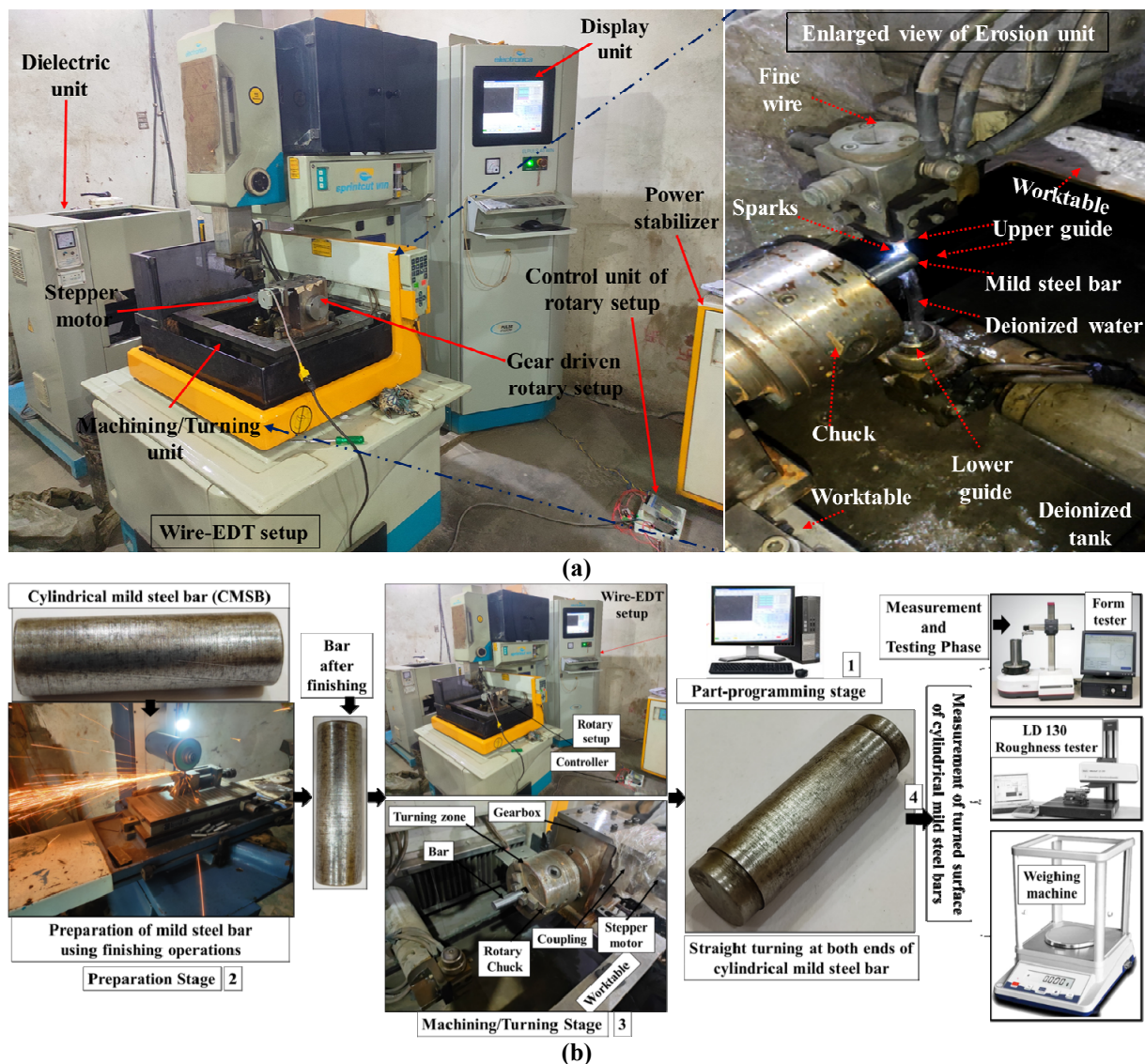
Figure 2. Wire-EDT machine setup used for straight turning and the procedure of turning cylindrical mild steel bars: (a) wire-EDT setup; and (b) turning procedure by wire-EDT.
