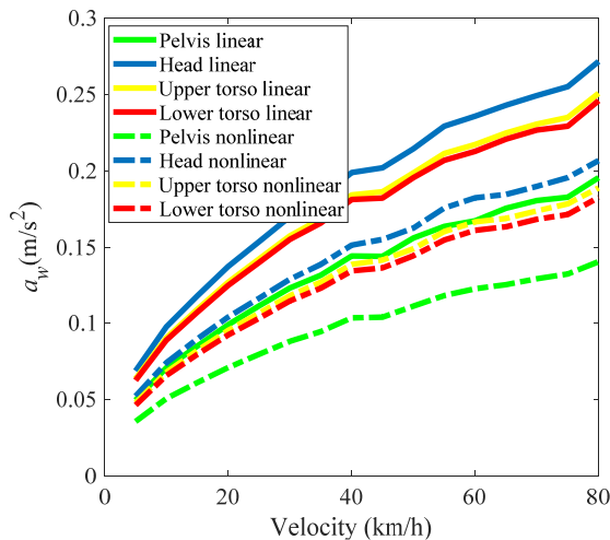
Figure 22. Body segments' RMS weighted acceleration (m/s 2 ) in the velocity domain
