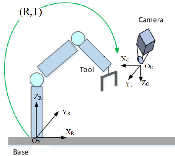
Figure 5. Robot and camera coordinate relation
