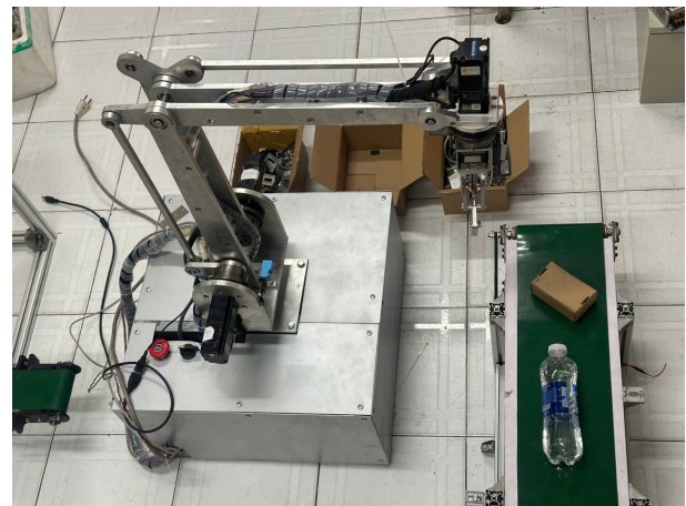
Figure 3. Practical system
