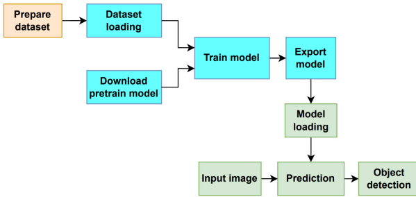
Figure 4. Flowchart to train the model for object detection
