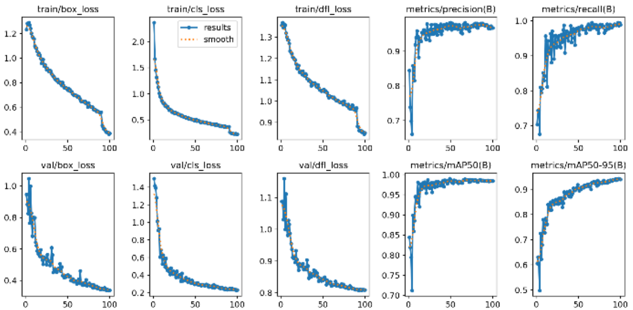
Figure 6. The training results for the YOLOv11 mode
