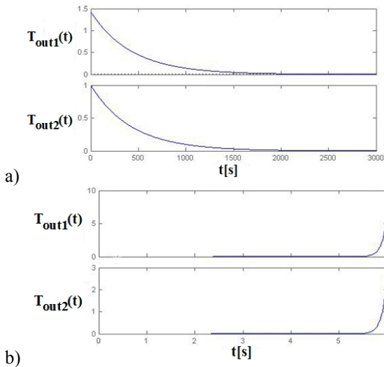
Figure 7. Simulation results for stability analysis: a) 2 wheels in contact inside the pipeline (on the drive part), b) 1 wheel in contact inside the pipeline (on the drive part)
