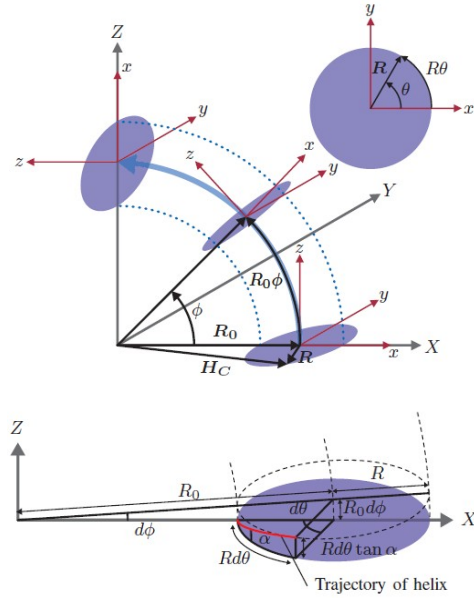
Figure 5. a) Display of parameters in the elbow, b) Elbow trajectory display
