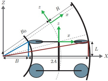
Figure 6. Display of robot motion through the elbow
