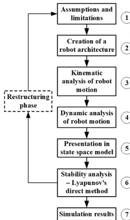
Figure 1. Diagrammatic representation of the approach to system stability testing
