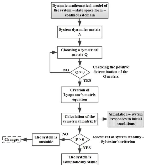
Figure 2. Diagrammatic representation of the stability analysis
