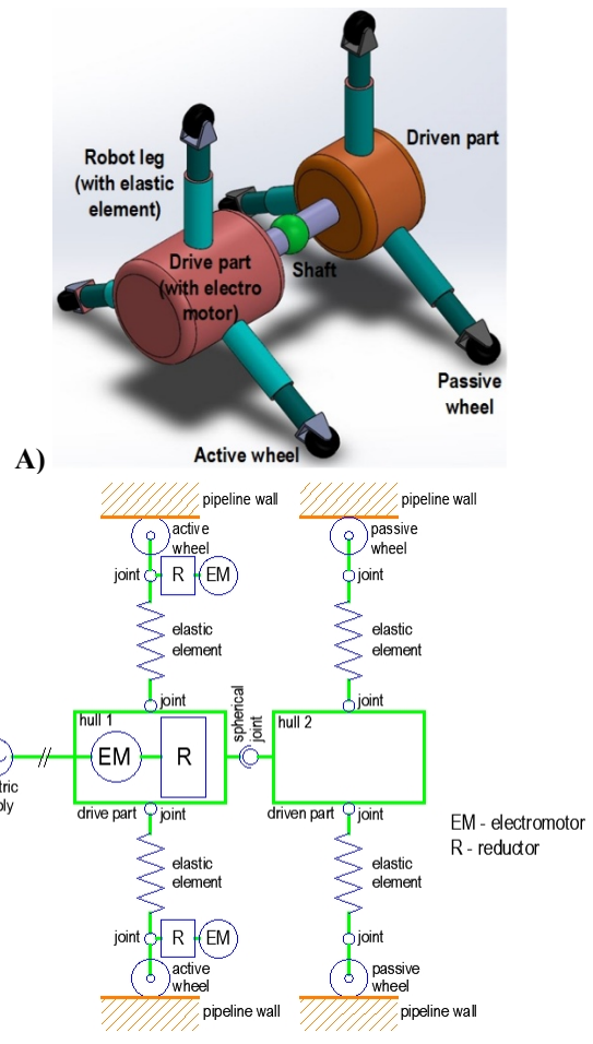
Figure 3. a) 3D Representation of the conceptual model of the architecture of the robotic system, b) Kinematical schema of the robotic system
