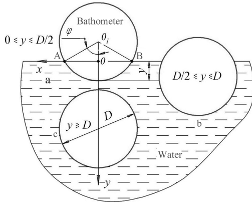
Figure 3. Stages of immersion of a bathometer in a body of water
