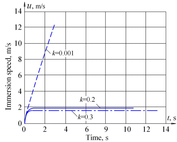
Figure 5. Dependence of the bathometer's sinking rate on time
