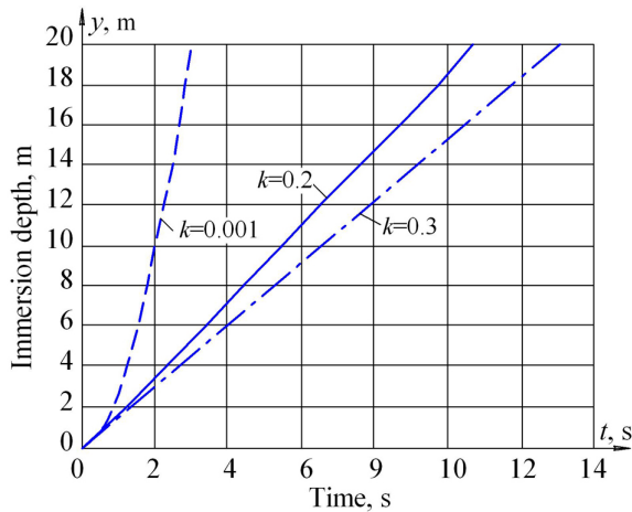
Figure 4. Dependence of the depth of immersion of the bathometer on time
