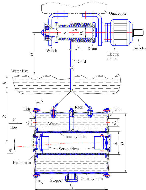
Figure 2. Design of drone technological equipment (See also A–A Figure 1)
