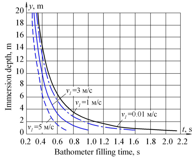
Figure 7. Dependence of the bathometer filling time on the immersion depth and the current speed in the reservoir
