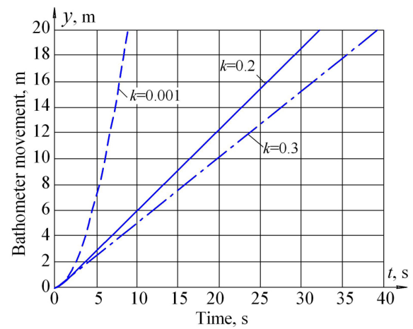
Figure 6. The trajectory of the bathometer
