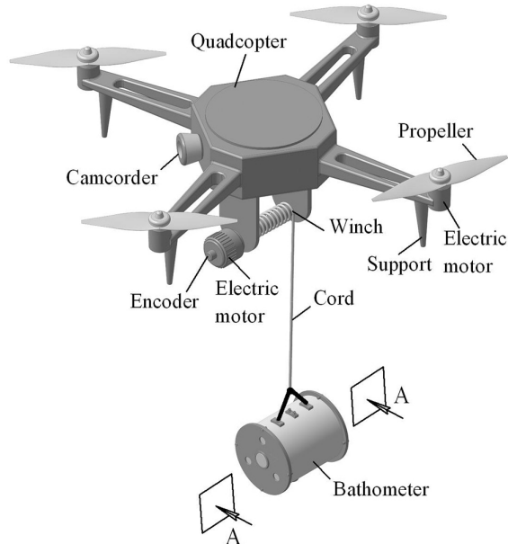
Figure 1. Drone for water sampling
