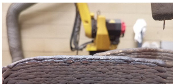
Figure 9. Multi-layers 3D structure wall using the optimal parameters
