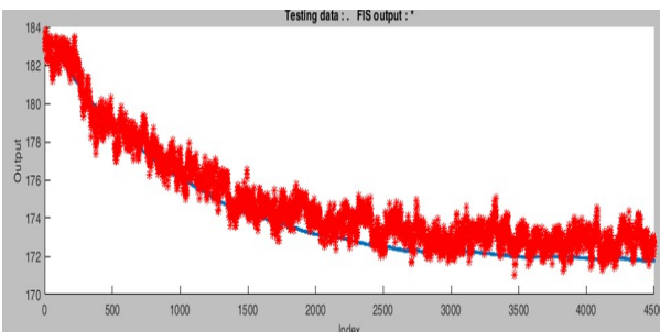
Figure 13. ANFIS Testing for Speed Control of DC Motor
