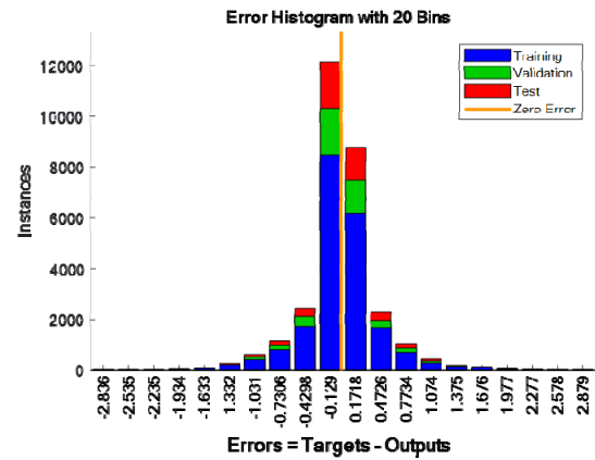
Figure 9. Error Histogram of ANN
