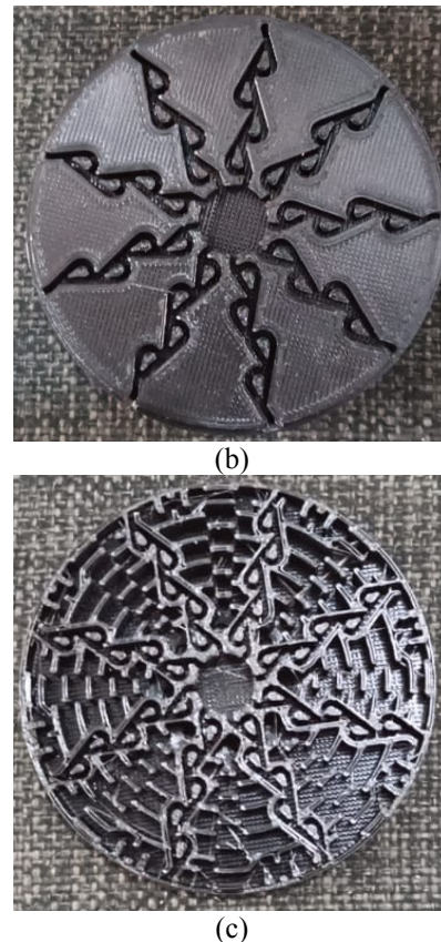
Figure 2. Sample 3D print Tesla Valve, a) cover inlet, b) based model, c) labyrinth model
