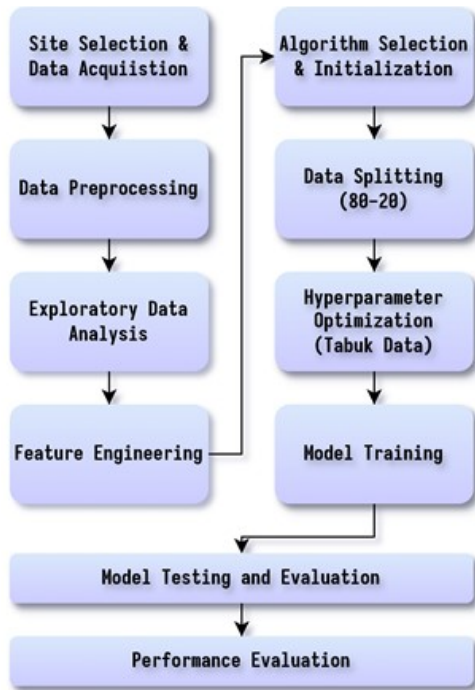
Figure 1. Methodological Flowchart
