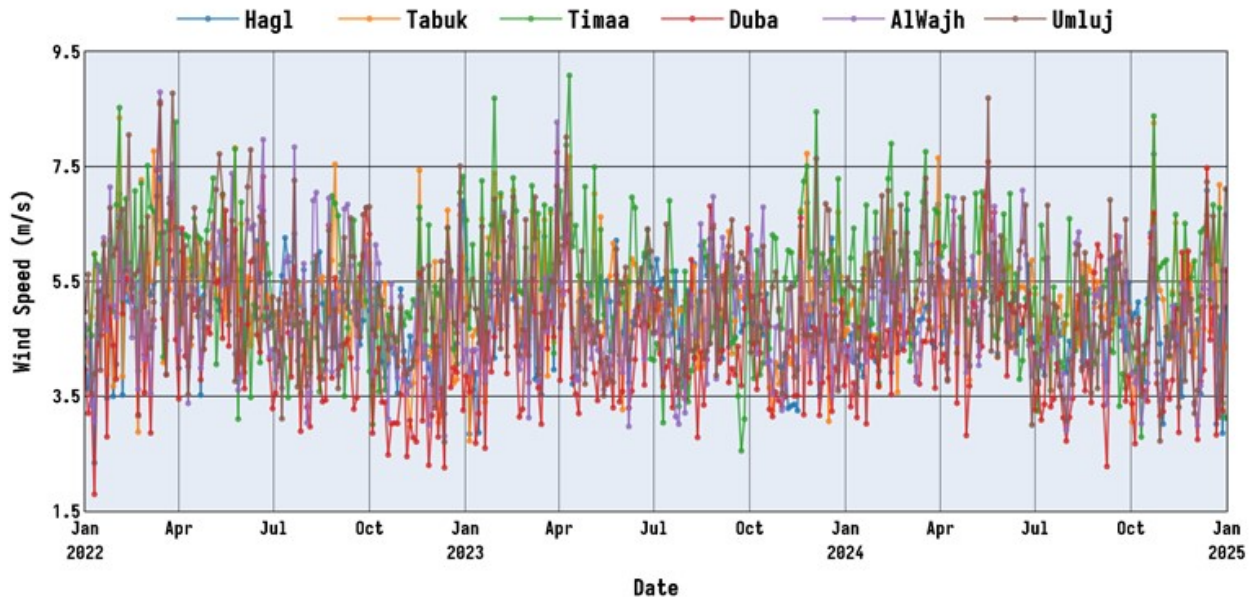
Figure 7: Wind Speed trends across chosen study sites
