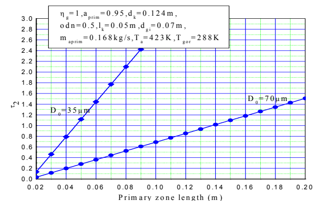
Figure 18. Parameter \tau_2 as a function of primary zone length at primary zone coefficient of the air excess 0.95, for droplet diameters 35 \mu\text{m} and 70 \mu\text{m} , regime 2
