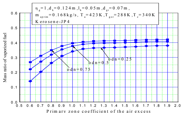
Figure 6. Mass ratio of the vaporized fuel as a function of primary zone coefficient of the air excess for different ratio of the air flows through vaporizer and primary zone, kerosene JP-4, regime 2
