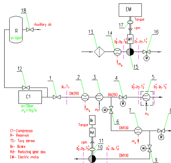
Figure 31. Laboratory scheme
