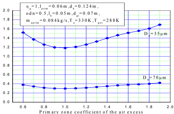
Figure 12. Parameter \tau_2 as a function of primary zone coefficient of the air excess for droplet diameters 35 \mu\text{m} and 70 \mu\text{m} , regime 1
