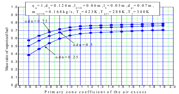
Figure 5. Mass ratio of the vaporized fuel as a function of primary zone coefficient of the air excess for different ratio of the air flows through vaporizer and primary zone, gasoline, regime 2
