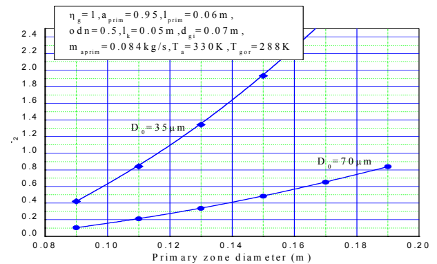
Figure 15. Parameter \tau_2 as a function of primary zone diameter at primary zone coefficient of the air excess 0.95, for droplet diameters 35 \mu\text{m} and 70 \mu\text{m} , regime 1
