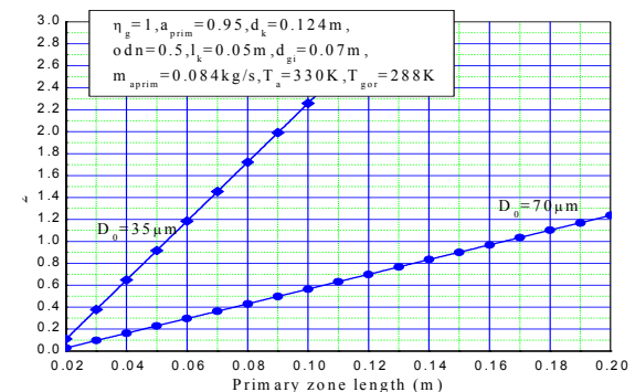
Figure 17. Parameter \tau_2 as a function of primary zone length at primary zone coefficient of the air excess 0.95, for droplet diameters 35 \mu\text{m} and 70 \mu\text{m} , regime 1
