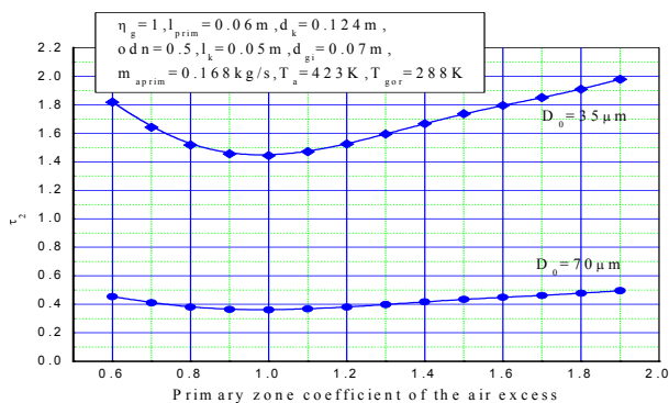
Figure 13. Parameter \tau_2 as a function of primary zone coefficient of the air excess for droplet diameters 35 \mu\text{m} and 70 \mu\text{m} , regime 2
