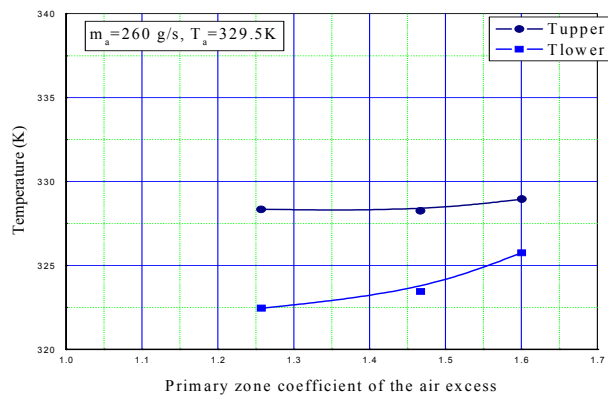
Figure 24. Temperature of the mixture at the vaporizer exit as a function of primary zone coefficient of the air excess, upper and lower half respectively
