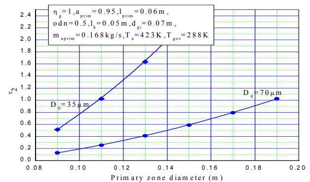
Figure 16. Parameter \tau_2 as a function of primary zone diameter at primary zone coefficient of the air excess 0.95, for droplet diameters 35 \mu\text{m} and 70 \mu\text{m} , regime 2
