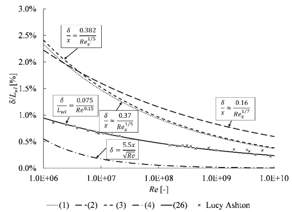
Figure 10. Non-dimensional boundary layer thickness change for different Re (1-4, 26)
