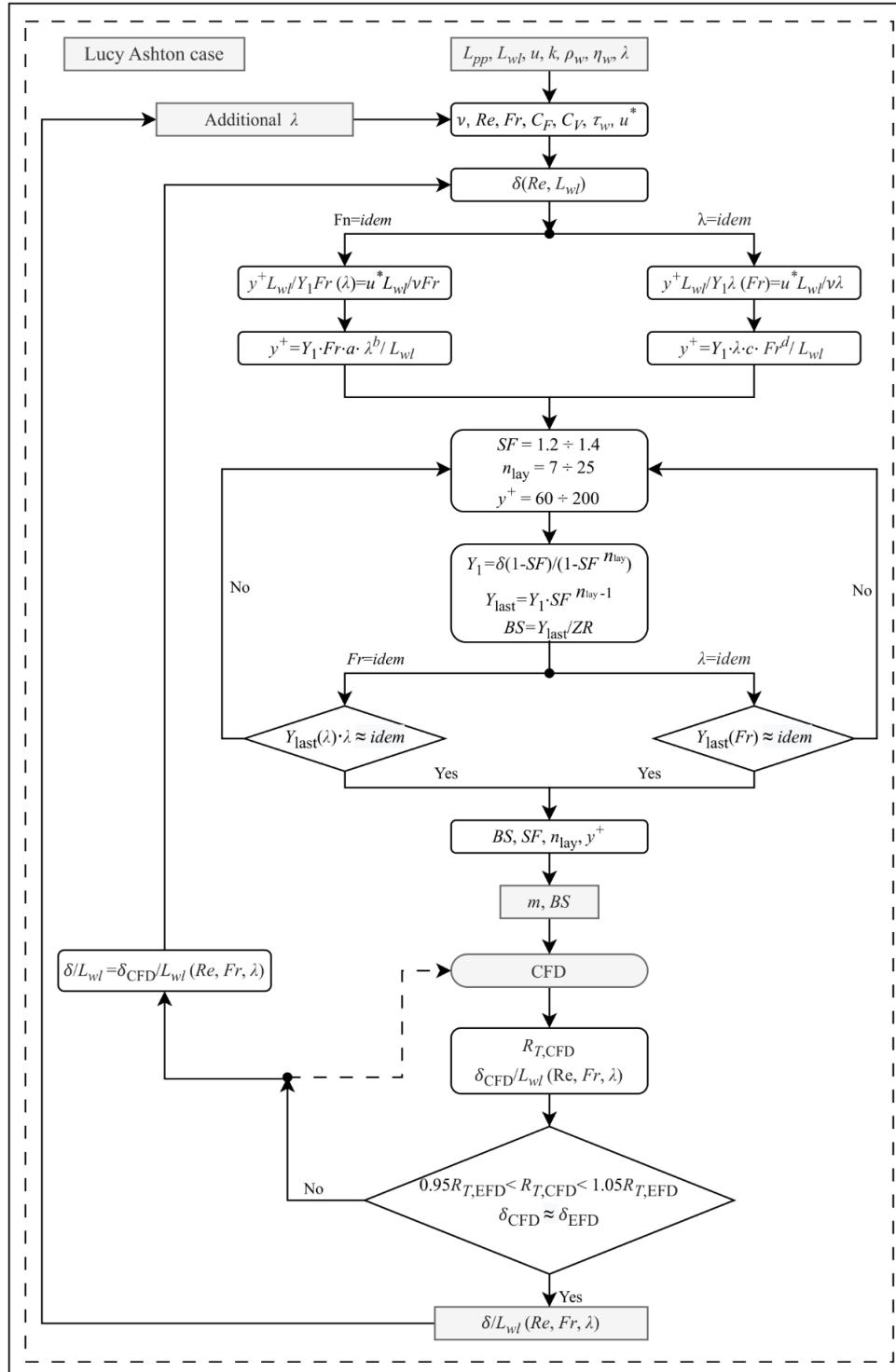
Figure 3. Methodology algorithm
