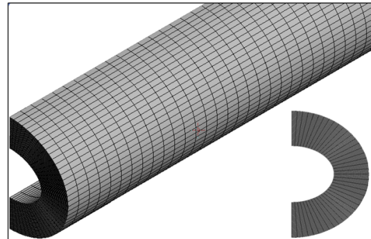
Figure 3. Optimal mesh. Case: Two ellipses: D_{oel-s}=1.8/ D_{oel-b}=2.2; D_{iel-s}=0.8/ D_{iel-b}=1.2
