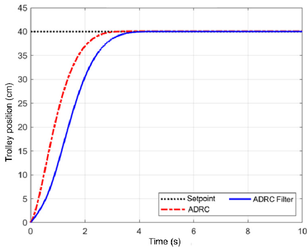
Figure 14. Trolley position response when m_P=2.2 kg
