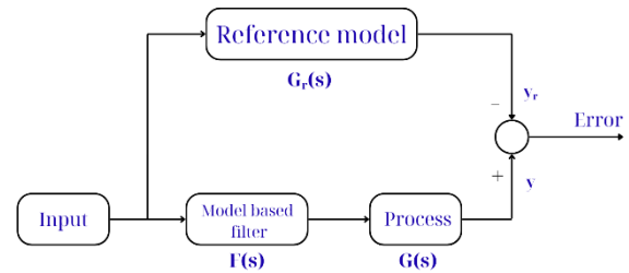
Figure 4. Model based Input filter design
