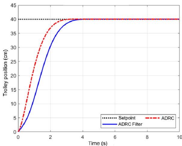
Figure 20. Trolley position response when l = 0.65 m
