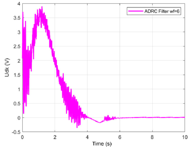
Figure 13. Control input voltage for \omega_f = 6
