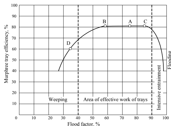
Figure A.1 General diagram of tray efficiency
