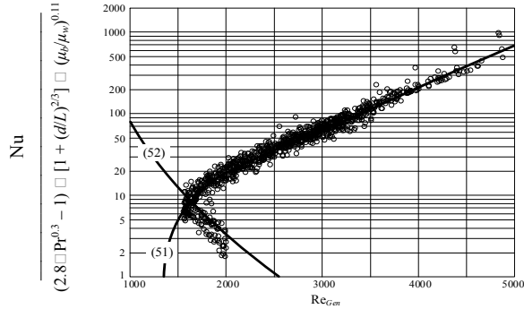
Figure 3 Nu vs. \text{Re}_{\text{Gen}} for regions B and C
