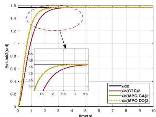
Figure 7. Performances of controllers for link 2
