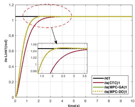
Figure 6. Performances of controllers for link 1
