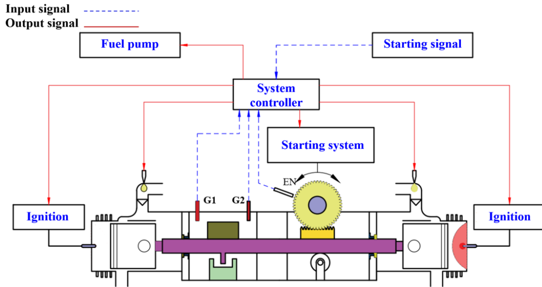
Figure 4. Schematic of the control system
