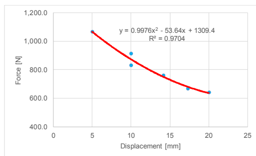
Figure 17. Force-equivalent crack length curve
