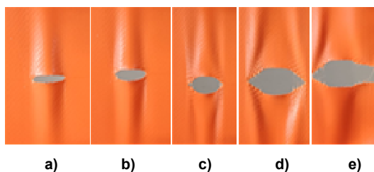
Figure 9. Crack propagation mechanism leading to final failure a) initial shape, b) elliptical shape, c) rupture of the first yarn, d) increase in the number of broken yarns, e) final rupture
