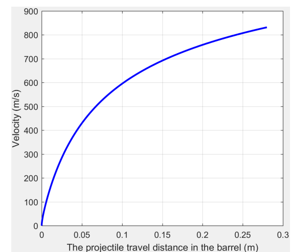
Figure 8. Projectile velocity.
