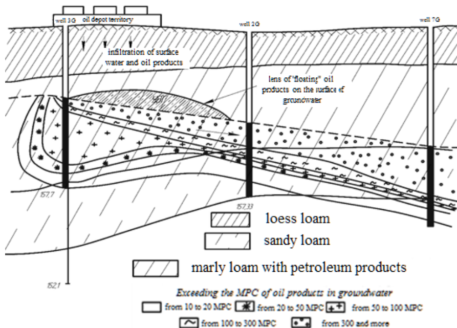
Figure 3: Schematic hydrogeological section in the area of the oil terminal
