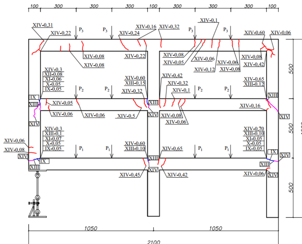
Fig. 6. Scheme of formation and width of cracks of all types in the RZh-2 frame structure after applying a special load
