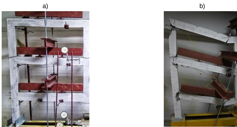
Fig. 7. The pattern of destruction in the experimental reinforced concrete frame-rod structural system after removing the central post with a prestressed crossbar above the first floor (a) and without a prestressed crossbar above the first floor (b)
