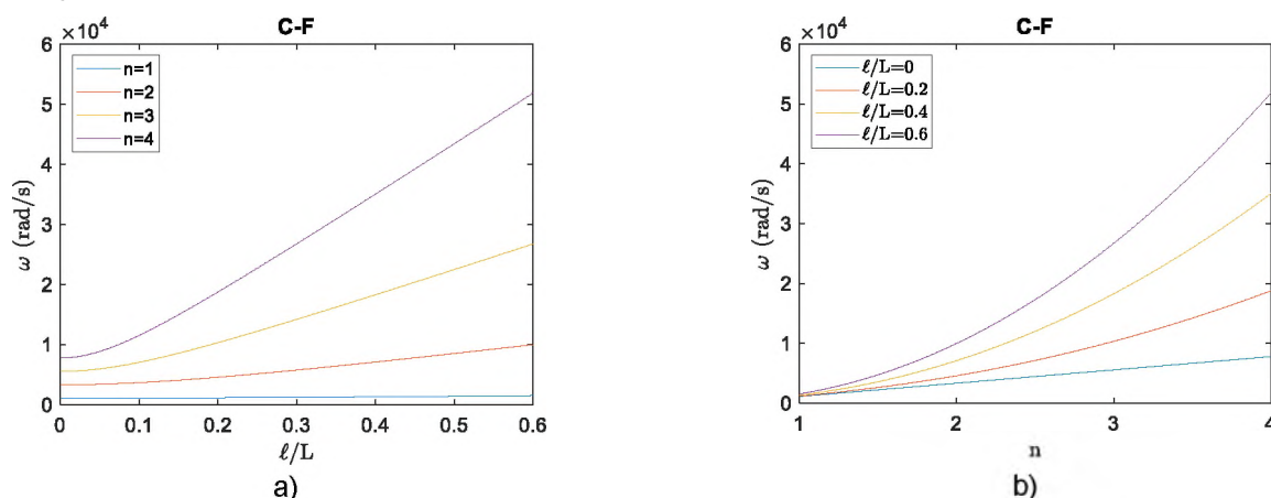
Fig. 2. Influence of the ratio \ell/L , and the mode number n , on the LF of the C-F GradEla bar
