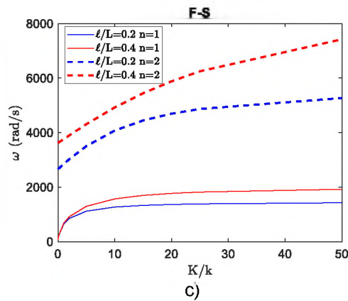
Fig. 9. Influence of the ratio \ell/L , the mode number n , and the ratio K/k , on the LFs of the F-S GradEla bar
