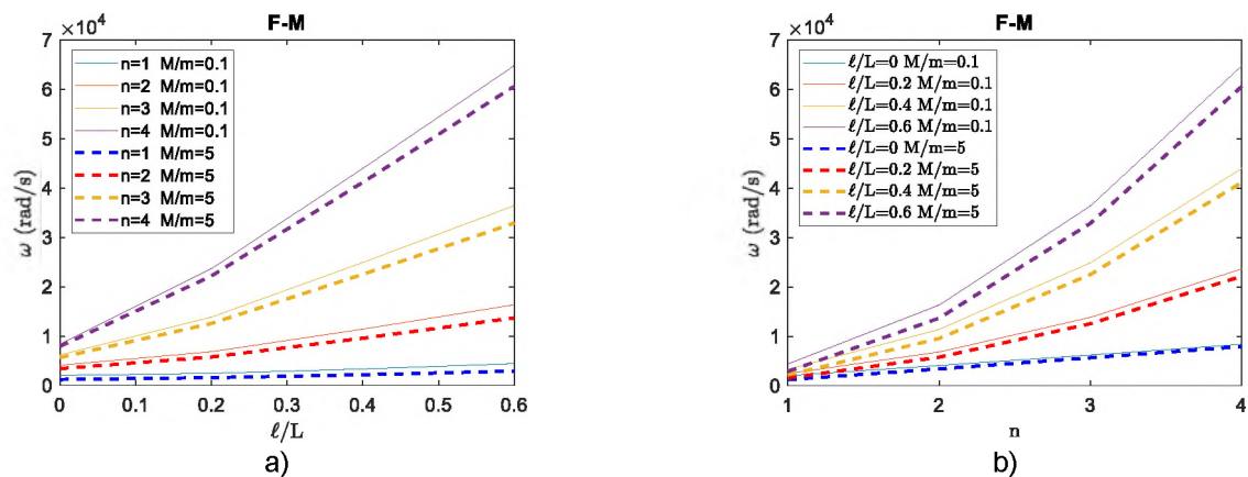
Fig. 7. Influence of the ratio \ell/L , the mode number n , and the ratios M/m and K/k , on the LFs of the C-MS GradEla bar
