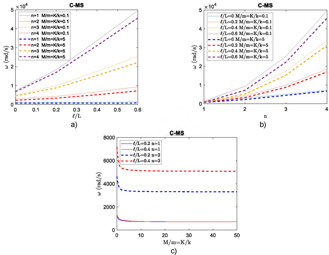
Fig. 7. Influence of the ratio \ell/L , the mode number n , and the ratios M/m and K/k , on the LFs of the C-MS GradEla bar
