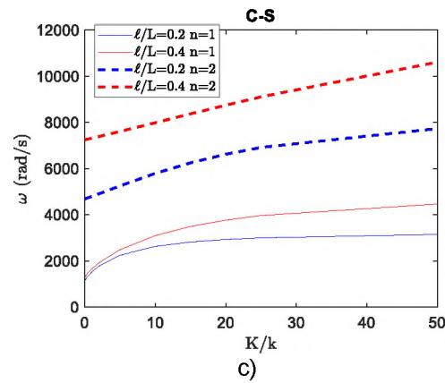
Fig. 6. Influence of the ratio \ell/L , the mode number n , and the ratio K/k , on the LFs of the C-S GradEla bar
