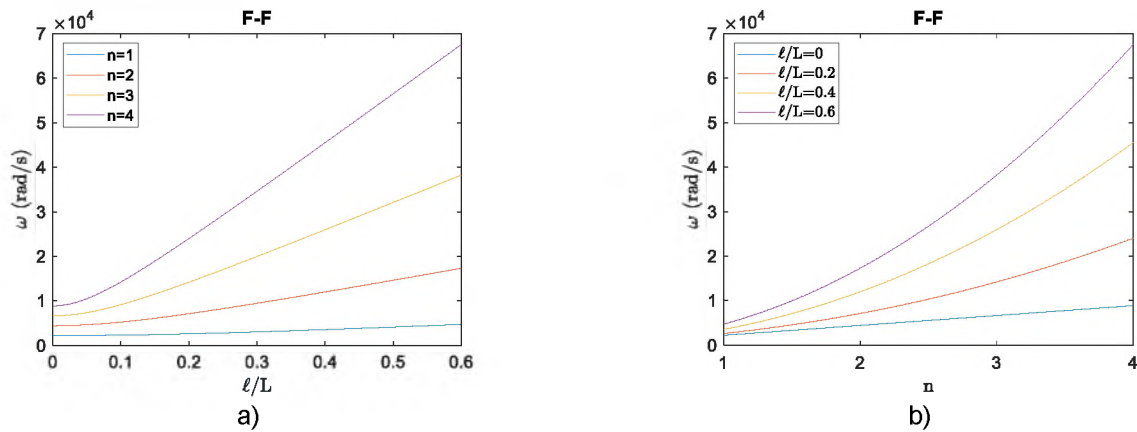
Fig. 4. Influence of the ratio \ell/L , and the mode number n , on the LFs of the F-F GradEla bar
