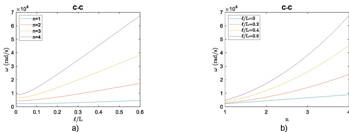
Fig. 3. Influence of the ratio \ell/L , and the mode number n , on the LF of the C-C GradEla bar
