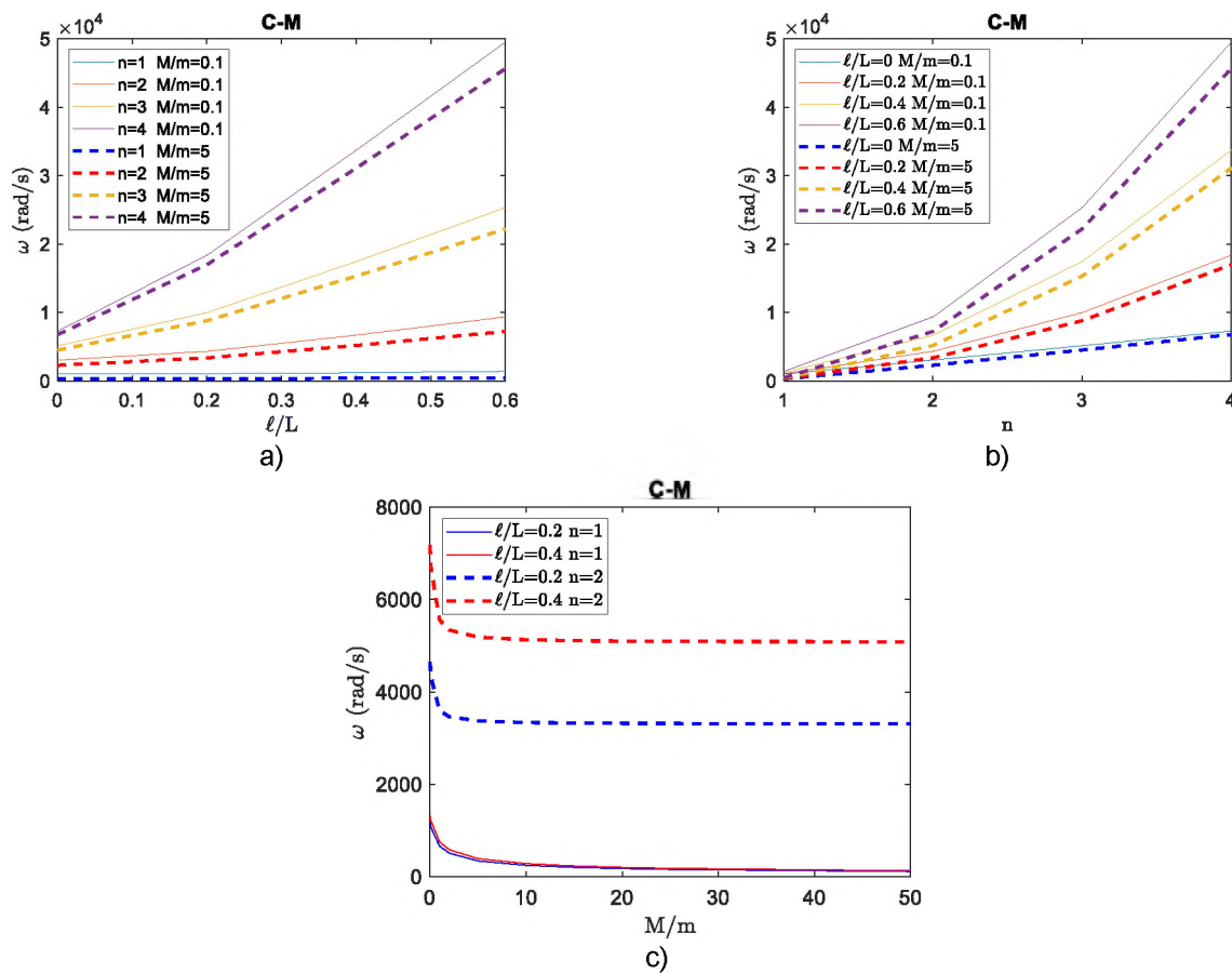
Fig. 5. Influence of the ratio \ell/L , the mode number n , and the ratio M/m , on the LFs of the C-M GradEla bar
