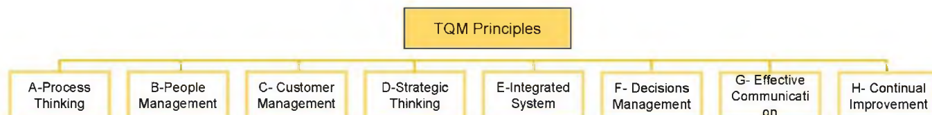
Fig 1. TQM principles [8]
