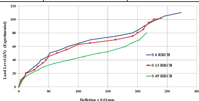
Fig.19. Load Level -Deflection Relationships for SRRCB (S6, S 13, S 45)
