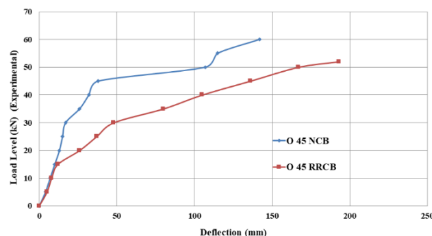
Fig.22 Load Level -Deflection Relationships for HRRCB &amp; NCB (O 45)
