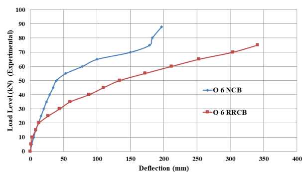
Fig.26. Load Level Carry Capacity-Deflection Relationships for HRRCB &amp; NCB (O6)
