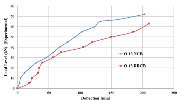
Fig.24. Load Level Carry Capacity -Deflection Relationships for HRRCB &amp; NCB (O13)
