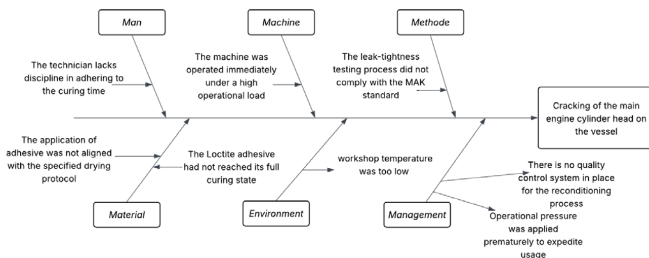
Fig. 3. Fishbone crack diagram
