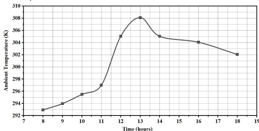
Fig. 4. Variation of ambient temperature with time for single and double-loop systems
