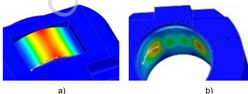
Fig. 12. Segments of the measurement results of the loads acting on the plate and the effect on the bushing housing, on the basis of which graphs of the pressure effect results were constructed: a) load measurement segment – from the lower part of the plate to its middle along an arc with a radius of 17 mm over a length of 10 mm; b) load measurement segment – along an arc from the minimum reaction to the maximum reaction on the inner surface of the bushing over a length of 10 mm
