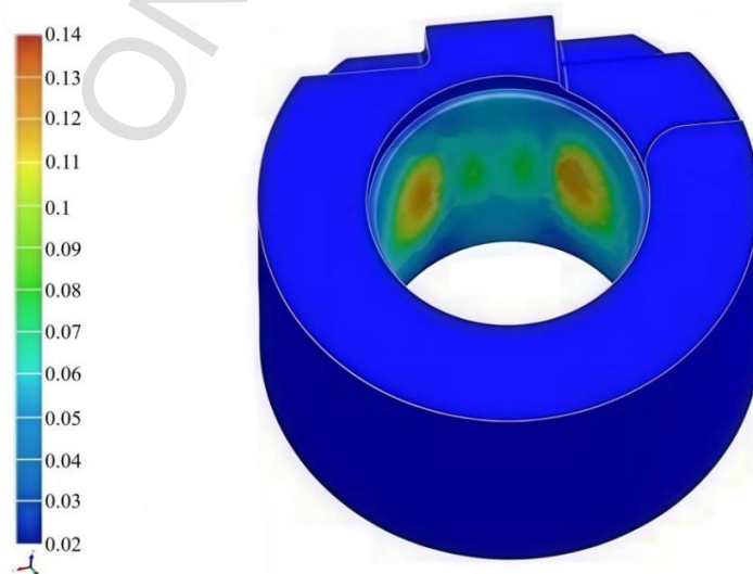
Fig. 15. Also shows a model displaying the reaction force of the plate acting on the bushing under a pressure load of 10 bar at 1000 rpm
