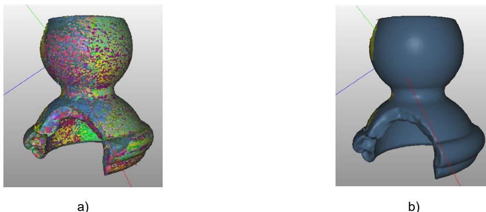
Fig. 5. Completely damaged articulated component: (a) point cloud obtained by 3D scanning; (b) generated mesh model prior to geometric reconstruction
