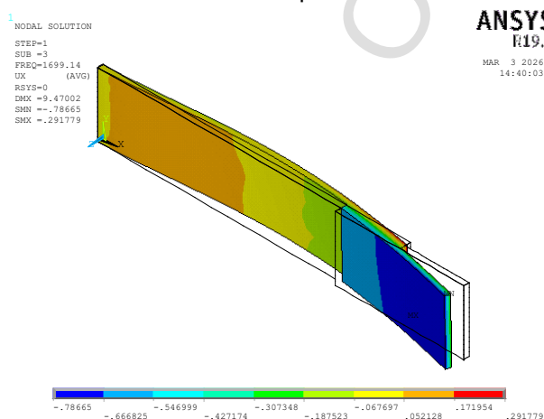
Mode shape -3-
