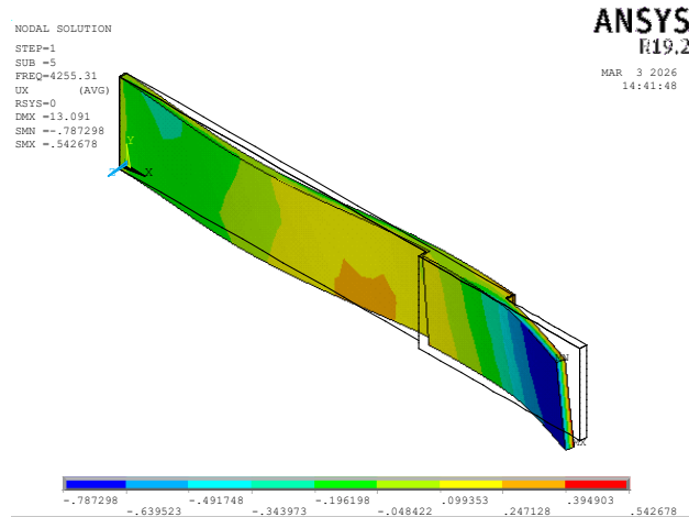
Mode shape -5-
