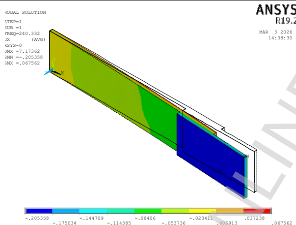
Mode shape -1-
