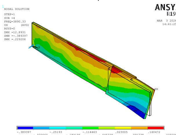
Mode shape -4-
