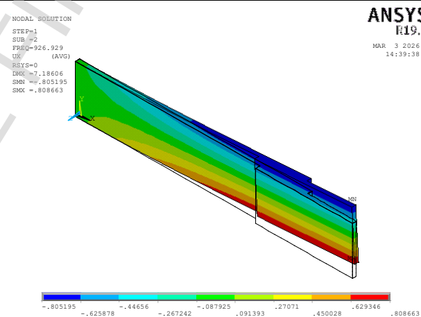
Mode shape -2-
