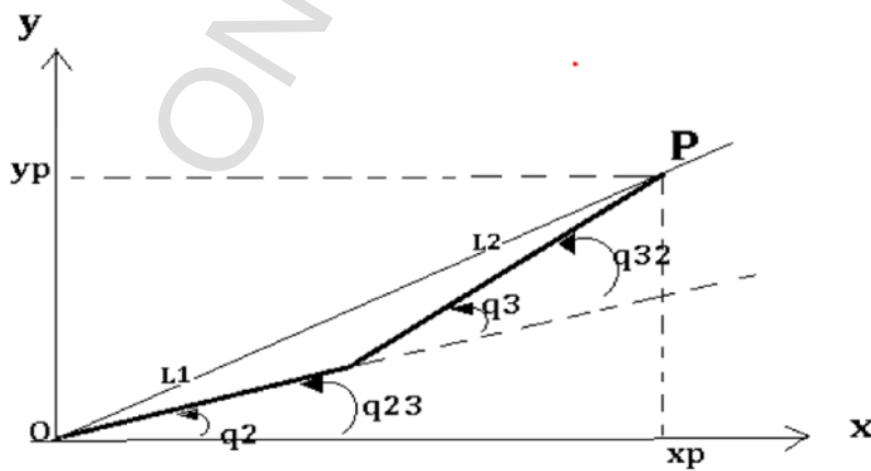
Fig. 2. Inverse kinematic diagram
