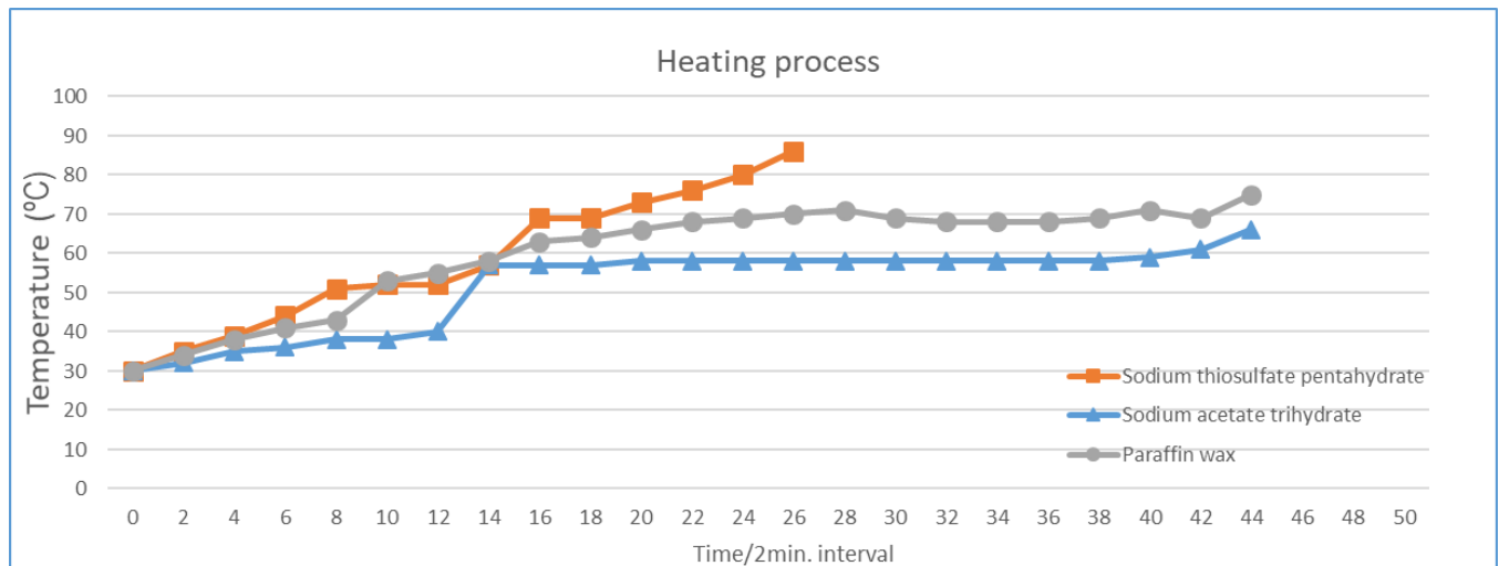
Fig. 3. Heating process
