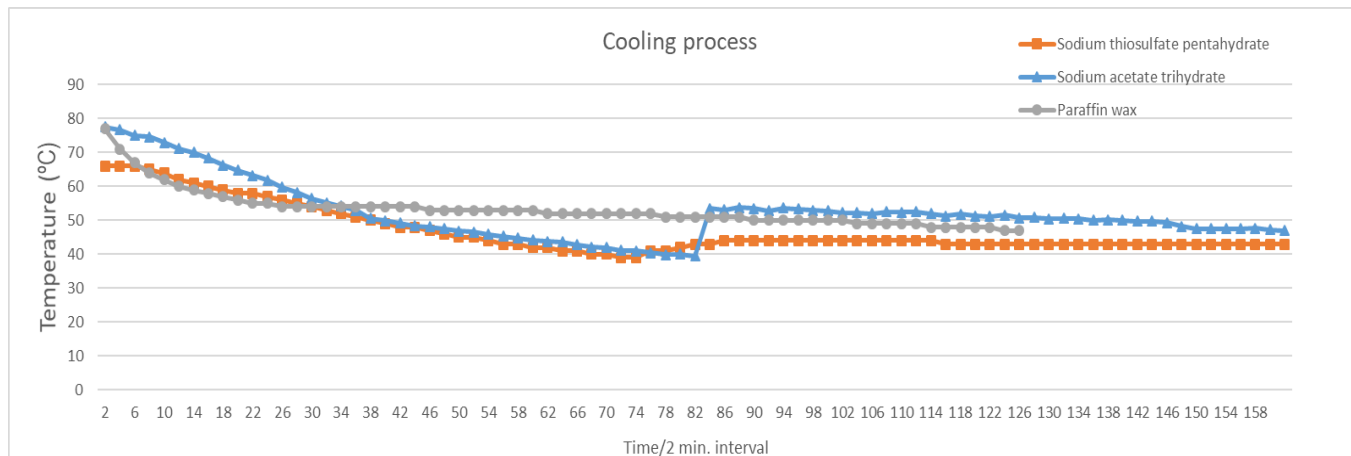
Fig. 4. Cooling process
