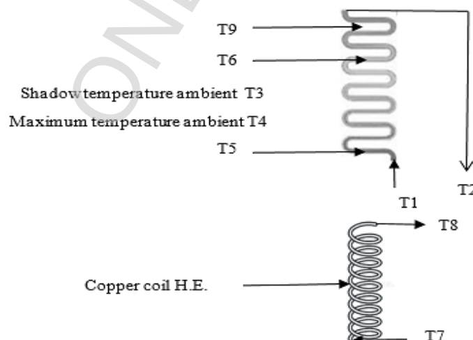
Fig. 2. Location of thermocouple on the Serpentine shape (condenser) behind the P.V. Panel and helical coil
