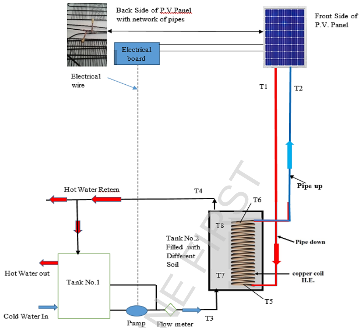
Fig. 1. Schematics of the experimental test rig
