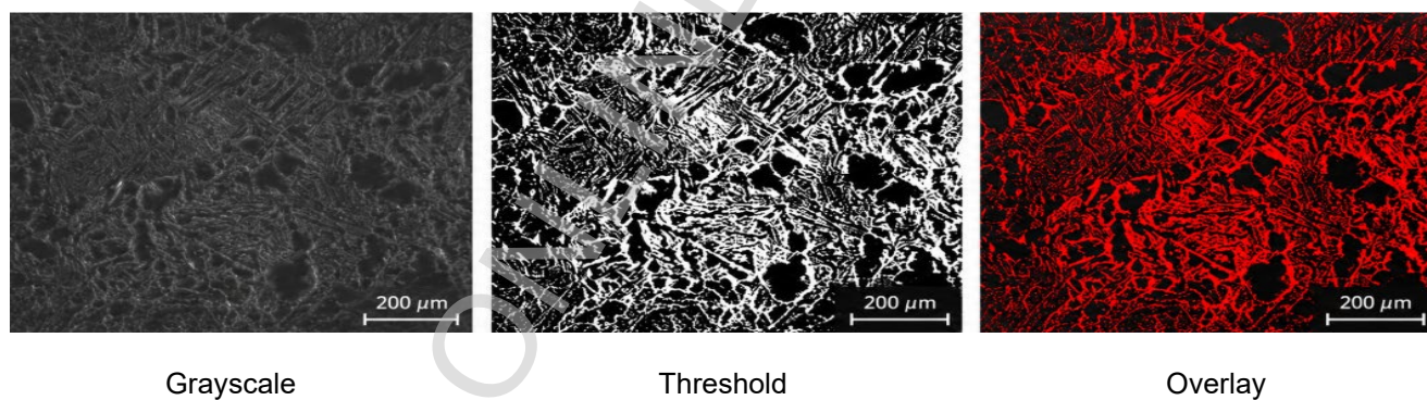
Fig. 15. Optical micrograph and ImageJ segmentation of the heat-affected zone at a welding speed of 60 cm/min using a 50× objective lens; scale bar = 200 μm
